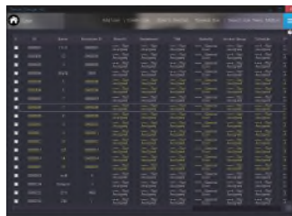
User Management
