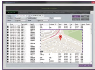
Log Management
